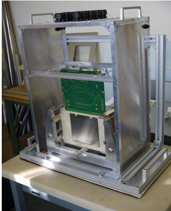
Figure 5.7: Photograph of the flexible mechanical structure. Tungsten absorber plates, glued on permaglass frames, are put into slots of the rod assembly.
