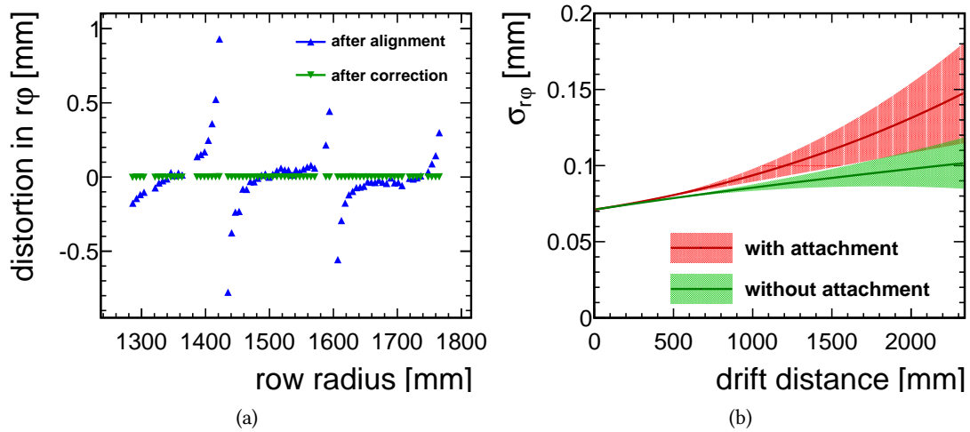
Figure 3.4: a) Alignment and distortion correction: mean hit position in r\varphi with respect to the track position at 1 T versus pad row radius. In blue after alignment correction, in green after distortion correction. b) Point resolution: extrapolation to a magnetic field of 3.5 T based on parameters measured with the Large TPC Prototype at 1.0 T. Plotted over the full ILD TPC drift length of 2.35 m including 1 error bands. In red with the measured attachment rate, in green without any attachment.
