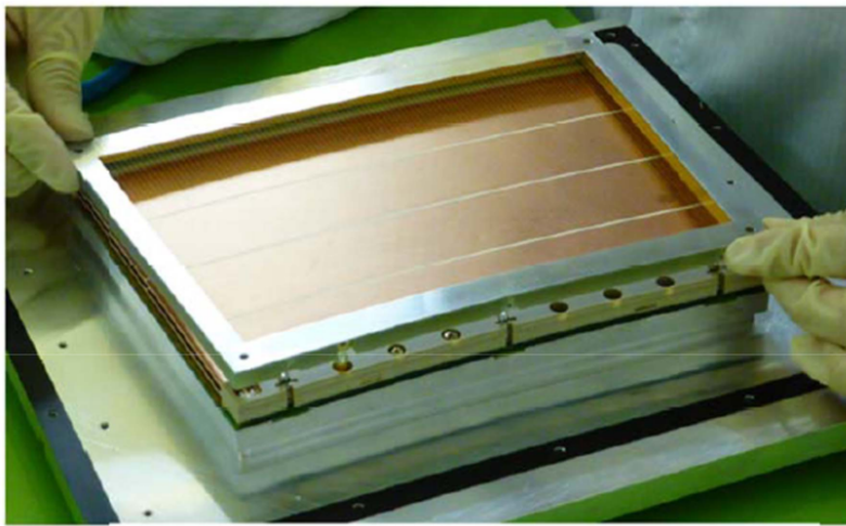
Figure 3.10: Prototype wire gate installed on the Asian GEM module.
