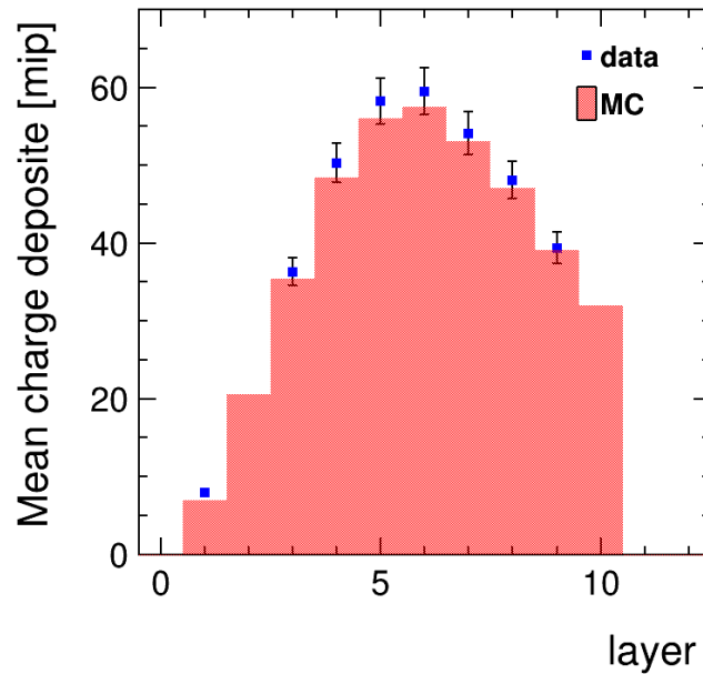
Figure 5.6: The mean charge read out for an electron shower as a function of the shower depth for data and Monte Carlo simulation. The mean charge is given in units of a mip response and the depth in units of a radiation length.
