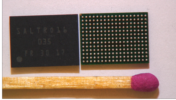
Figure 3.15: Photograph of two SALTRO-16 chip side-by-side and a matchstick for comparison.
