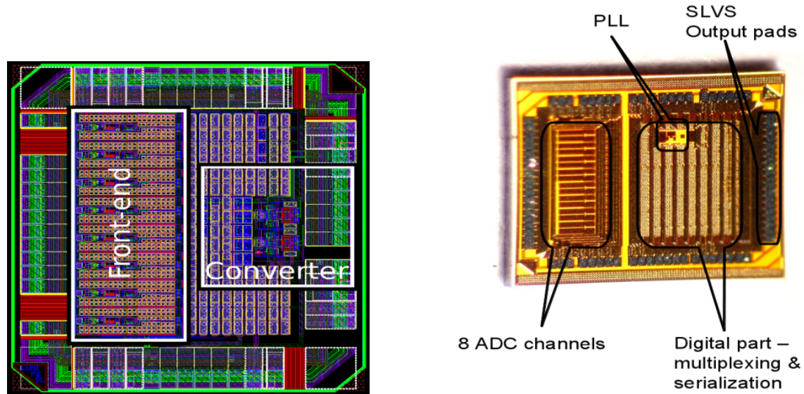
Figure 5.8: Left: 8 channel FE ASIC in 130 nm technology. Right: ADC ASIC in 130 nm technology.
