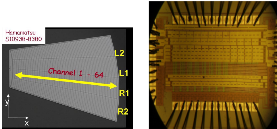
Figure 5.3: Left: LumiCal Sensors. Right: LumiCal ASIC
