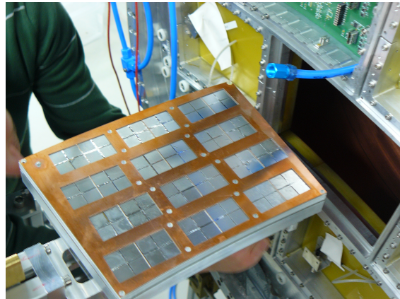
Figure 3.8: Fully equipped module as it is being mounted
