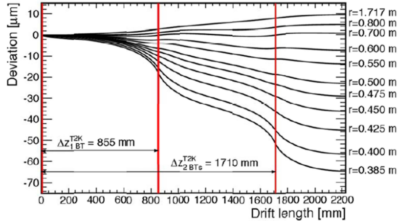
Figure 3.9: Displacement due to the positive-ion discs.
