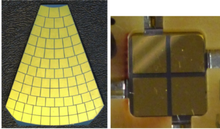
Figure 5.2: Left: A GaAs pad sensor developed for BeamCal. Right: CVD diamond sensors
