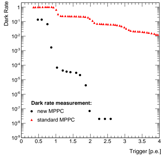
Figure 4.11: Dark count rate of recent SiPMs, MPPC devices by Hamamatsu, without (standard) and with (new) inter-pixel cross talk suppression. ( Courtesy MPI for Physics, Munich )
