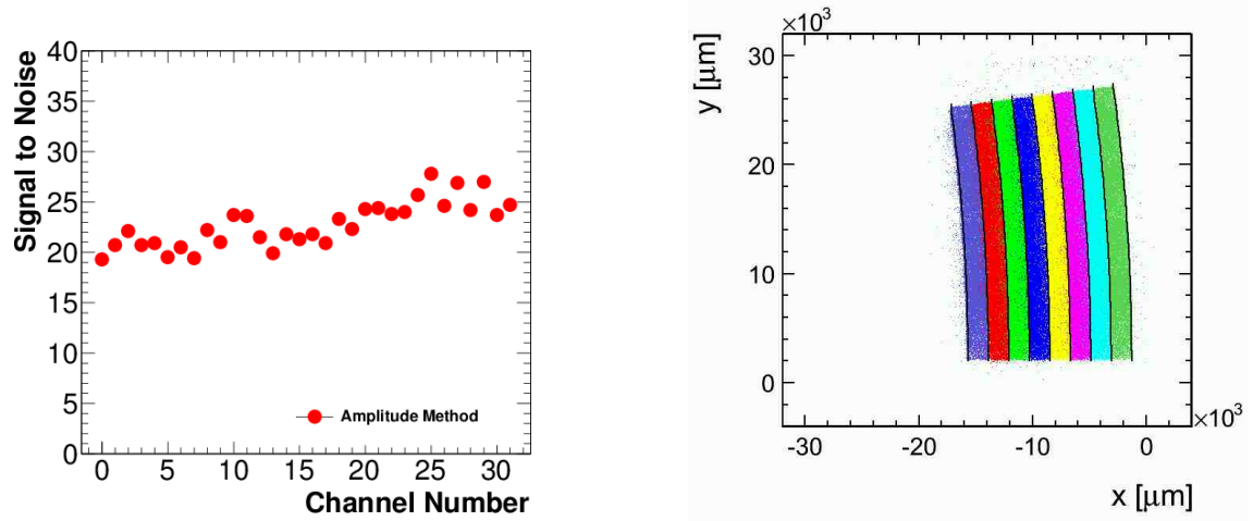
Figure 5.5: Left: The signal-to-noise ratio of all readout channels. Right: Distribution of the predicted impact points on pads with a color coded signal.
