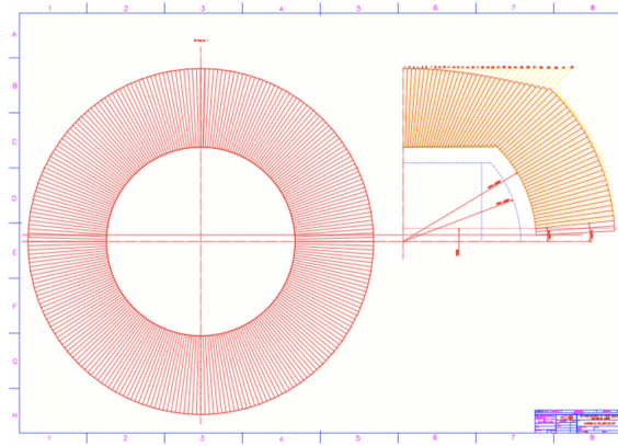
Figure 4.48: The 4th Concept [160] calorimeter geometry. This geometry was fully simulated.
