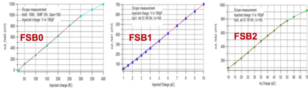
Figure 4.27: Dynamic range of the fast shapers associated to the three thresholds of the new version of HARDROC.
