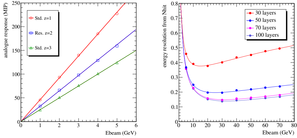
Figure 4.41: Electron response of a virtual Micromegas SDHCAL deduced from measurements of longitudinal shower profiles in non-resistive ( z=1 and z=3 ) and resistive ( z=2 ) Micromegas prototypes placed behind increasing thicknesses of passive material (left). Geant4 calculation of the energy resolution to pions of a Micromegas DHCAL of 30 to 100 layers based on simple hit counting (right).
