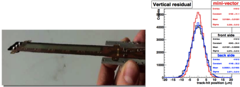
Figure 1.1: left: Photograph of a MIMOSA ladder for EUDET. right: A track resolution of 3\text{ }\mu\text{m} has been achieved.
