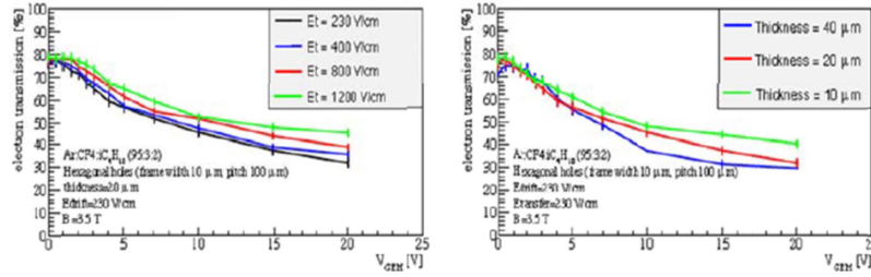
Figure 3.11: The electron transmission simulated for a gate-GEM with the honeycomb-shaped holes of pitch 100 \mu\text{m} and rim width 10 \mu\text{m} .
