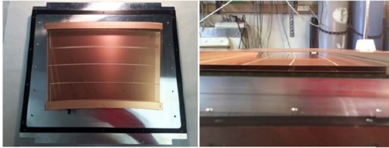
Figure 3.14: Left panel: Test mounting of the gate-GEM. Right panel: Test assembly of the gate GEM on the Asian GEM module.
