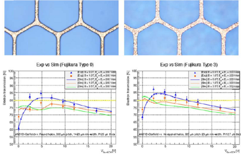
Figure 3.12: Upper: Honeycomb hole structure of the gate-GEM. The pitch of the holes is 335 \mu\text{m} , the rim width 29 \mu\text{m} . The polyimide insulator is 12.7 \mu\text{m} thick. Lower: Preliminary results of the electron transmission measurement are compared to simulation as functions of the GEM voltage for two types of gate-GEMs. In the left panel are results for gate-GEM with round holes; in the right panel results for the gate-GEM with the honeycomb-shaped holes.
