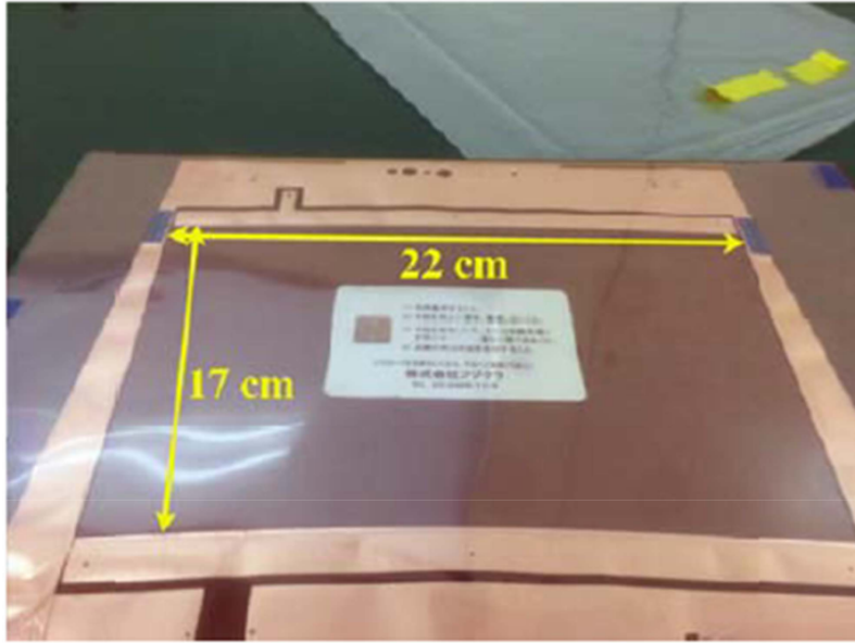
Figure 3.13: A sample gate-GEM for the Asian module.
