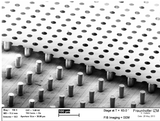
Figure 3.7: GridPix detector with a partially removed grid
