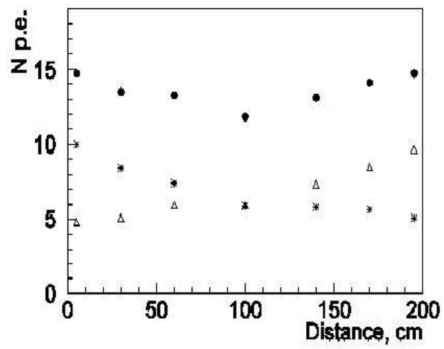
Figure 6.2: Sensitive Layers of ILD Muon /Tail Catcher Detector and number of detected photons
