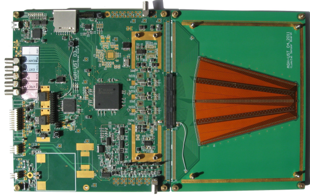
Figure 5.4: Photograph of a fully instrumented detector plane for FCAL.
